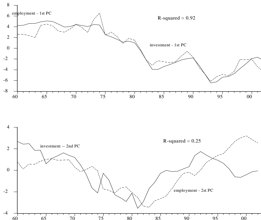
Figure 1. The first two principal components.
