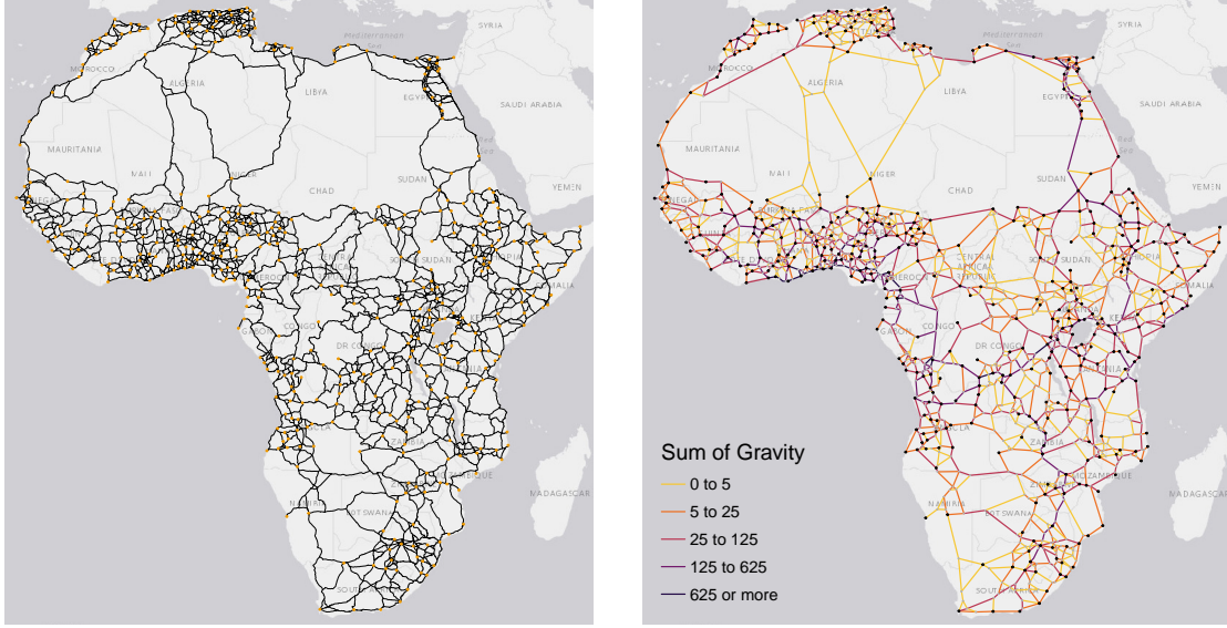
Figure 12: Computing an Optimal Graph of Africa's Transport Network
